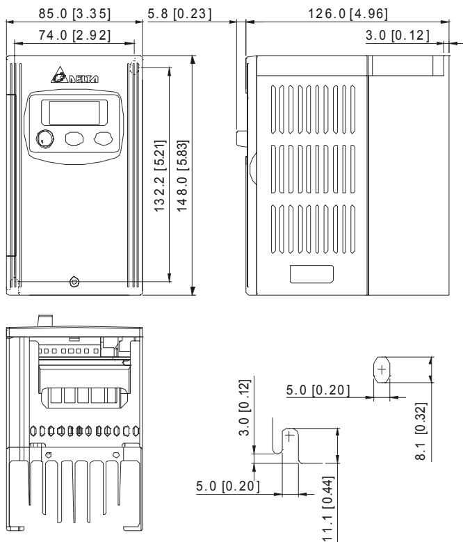
Frame S1: VFD004S43A, VFD004S43E, VFD007S43A, VFD007S43E
