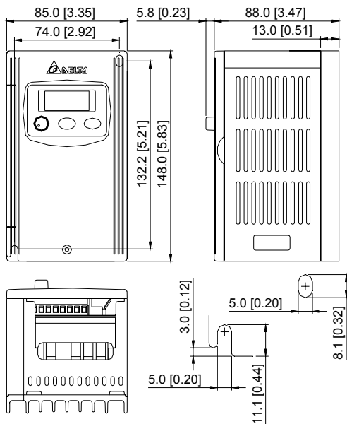
Frame S1: VFD002S11A, VFD002S21A, VFD002S23A
